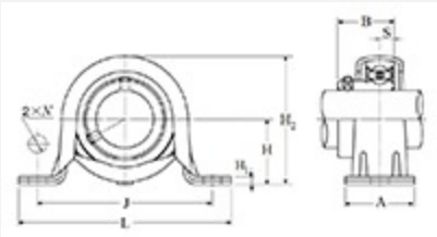
Pillow Block Unit, Set Screw, Pressed Steel Housing, ASPP Type - Dimensions
