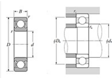
Single Row Radial Ball Bearing - Double Sealed (Contact Rubber Seal) - Dimensions
