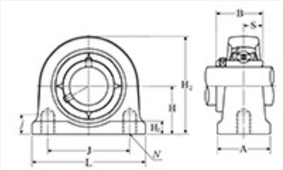
Pillow Block Unit, Set Screw, Narrow Style, UCUP Type - Dimensions
